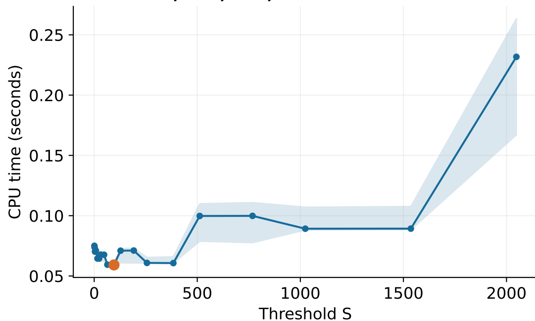
n = 1,000,000; coarse winner S=96
