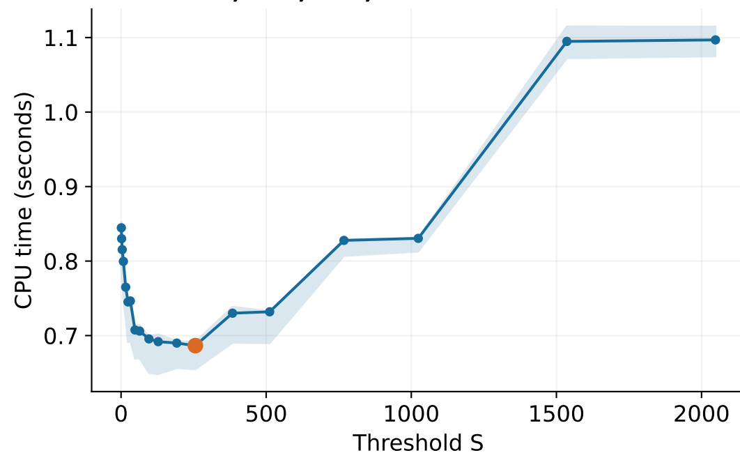
n = 10,000,000; coarse winner S=256
